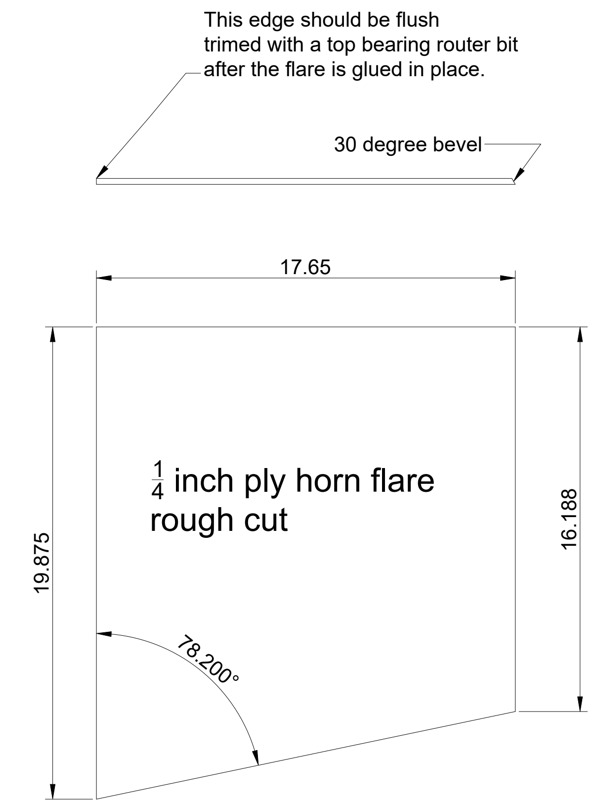
Altec A7 Horn Flare cut details.
